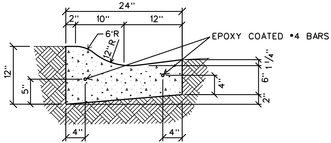
MOUNTABLE CURB DETAIL
