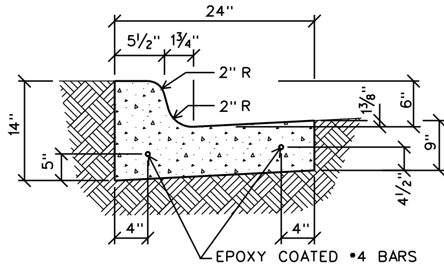
STANDARD CURB & GUTTER DETAIL
